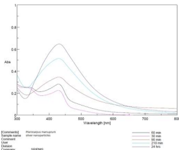
Figure 6: Uv-visible absorption spectra of silver nanoparticles at different intervals
