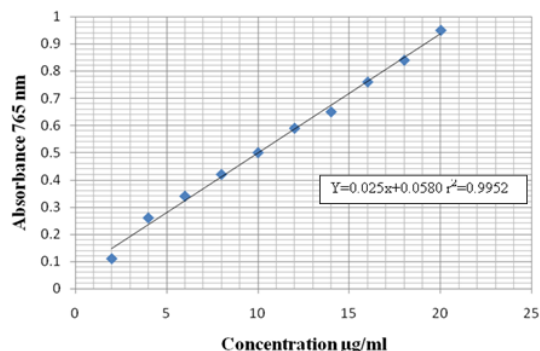
Figure 4: Calibration curve of Gallic acid.
